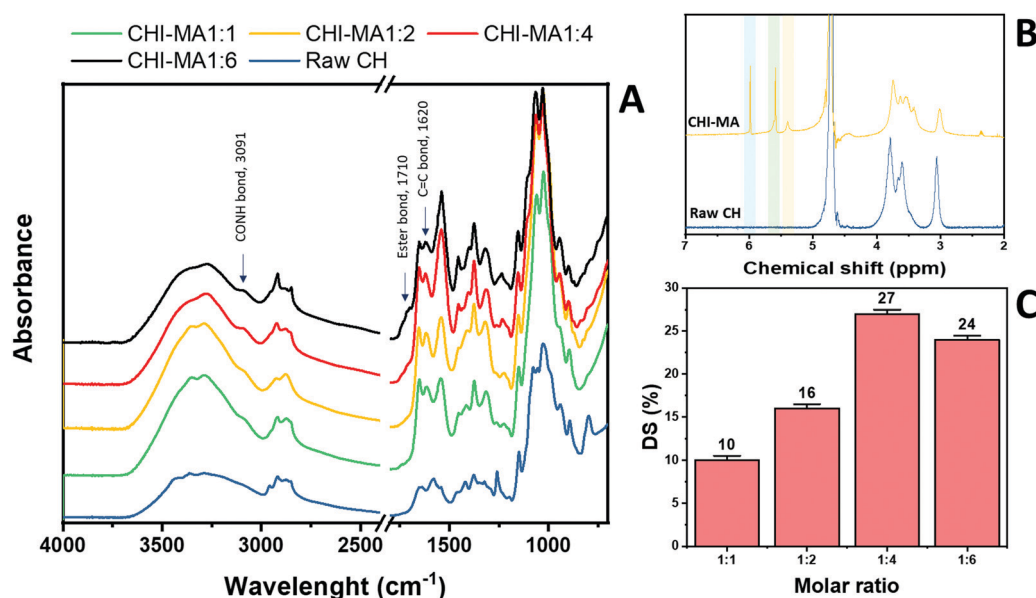
Fig. 2 FTIR spectra of raw chitosan and CHI-MA at different ratios of MA (A) and ^1\text{H-NMR} of CHI-MA (B). Degree of methacrylation of the samples prepared at different ratios of MA (C).
