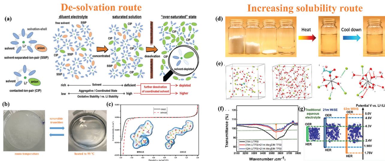
Fig. 15 (a) Design idea of further depletion of solvent molecules in the \text{Li}^+ solvation sheath. 260 (b) Optical images of top view of OSGE at RT and 95^\circ\text{C} . 55 (c) Comparison of ESW and \text{Li}^+ solvation sheath between OSGE and RTSGE. 55 (d) WSOE 45-1 prepared by stoichiometric amounts of \text{ZnCl}_2 , \text{ZnBr}_2 , \text{Zn}(\text{OAc})_2 , and water. 263 (e) Snapshots and extracted typical molecules conformations of MD simulation on WSOE 45-1 and 5 m \text{ZnBr}_{0.5}\text{Cl}_{1.5} aqueous solution. 263 (f) FTIR spectra of WiSE, 42 m WiHS, and 63 m WiHS electrolytes. 220 (g) MD simulation results and ESWs of traditional aqueous electrolyte, WiSE and WiHS electrolyte. 220
