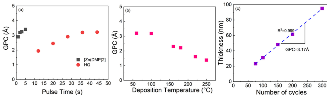
Fig. 5 ALD/MLD characteristics for the [\text{Zn}(\text{DMP})_2] + \text{HQ} process on Si(100): (a) saturation study with individually increased precursor pulse lengths, the other pulse length was fixed at 36 s and 2 s for HQ and [\text{Zn}(\text{DMP})_2] , respectively, (b) GPC versus deposition temperature behavior, and (c) linear dependence of film thickness on the number of ALD/MLD cycles applied; in (a) and (c), deposition temperature was 60 °C, in (b) & (c) pulse/purge sequence was: 2 s [\text{Zn}(\text{DMP})_2] /15 s \text{N}_2 /36 s HQ/80 s \text{N}_2 .
