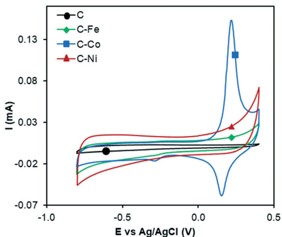
Fig. 6 Cyclic voltammograms in \text{N}_2 -saturated KOH solution at 1000 rpm and 50 \text{ mV s}^{-1} of C, C-Fe, C-Co and C-Ni.
