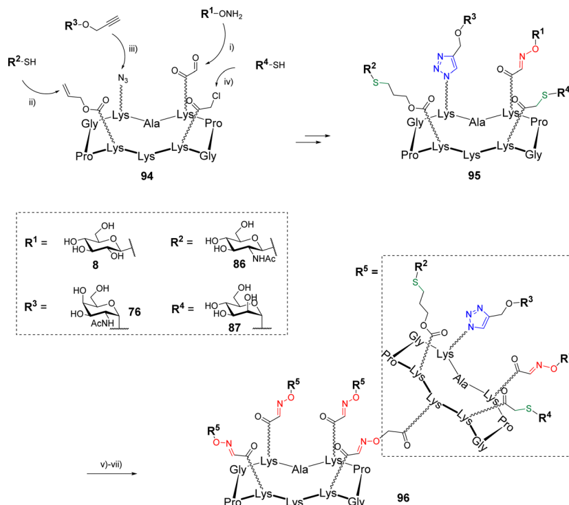
Scheme 19 Sequential one-pot synthesis of the heterovalent glycocluster 95 using four conjugation strategies and assembly of the glycodendrimer 96 . Reagents and conditions: (i) 0.1% TFA in \text{H}_2\text{O} , r.t., 30 min; (ii) DPAP, DMF/ \text{H}_2\text{O} , irradiation, 365 nm, r.t., 30 min; (iii) \text{CuSO}_4 , THPTA, sodium ascorbate, DMF/PBS (1 : 1, pH 7.4), r.t., 1 h; (iv) KI, DMF/ \text{H}_2\text{O} (1 : 1), DIPEA, r.t., 1 h; 47% over four steps; (v) N -succinimidyl (Boc-aminoxy)acetate, DIPEA, DMF; (vi) 50% TFA in \text{CH}_2\text{Cl}_2 , r.t., 30 min, 93% over two steps; (vii) 51 , 0.1% TFA in \text{H}_2\text{O} , 37 °C, 30 min, 87%.
