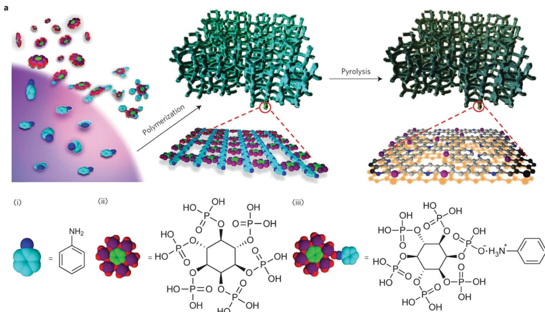
Fig. 97 (a) Schematic illustration of the preparation process for the NPC foams. An aniline (i)–phytic acid (ii) complex (iii) is formed (for clarity, only one of the complexed anilines is shown for an individual phytic acid), followed by oxidative polymerisation into a three-dimensional PANi hydrogel crosslinked with phytic acids. For clarity, only a piece of the two-dimensional network building block is shown in the enlarged view under the three-dimensional PANi hydrogel and only a piece of the two-dimensional NPC network building block is shown in the enlarged view under the three-dimensional NPC). Reproduced with permission from ref. 1389 Copyright Nature Publishing 2015.
