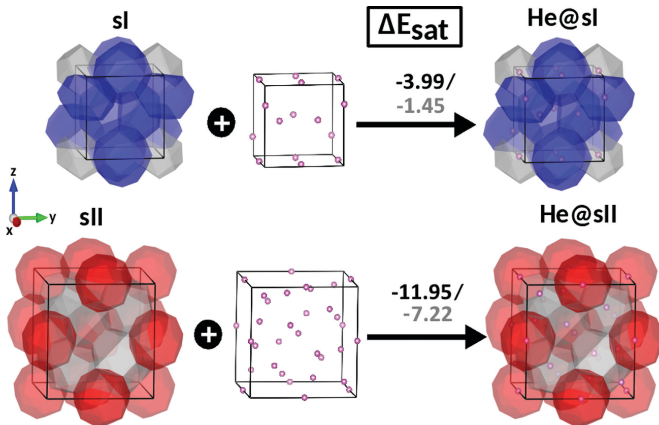
Fig. 5 Saturation energies, \Delta E_{\text{sat}} , in kcal mol -1 , for fully single cage occupation He@sI and He@sII clathrate hydrates, as computed from the present PW86PBE-XDM/D4 calculations.
