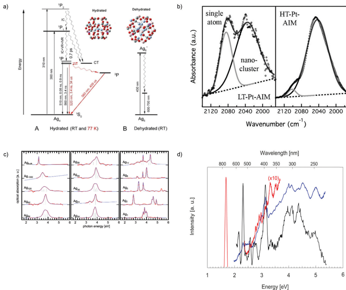
Fig. 11 (a) Ag clusters (AgCLs) confined within Na-exchanged Linde type A zeolites show dependence of luminescence lifetime on the water content indicating a possible way to speed or delay the electron–hole recombination in a controlled way. Proposed simplified kinetic scheme of the processes observed upon excitation of hydrated (A) and dehydrated (B) samples. The processes depicted in black and red are observed at RT and 77 K, respectively. (b) Single atoms and few-atom clusters of platinum exhibit high catalytic activity for ethylene hydrogenation while exhibiting resistance to sintering up to 200 °C. In situ IR spectroscopy reveals the presence of both single atoms and few-atom clusters that depend upon synthesis conditions. IR spectra of CO adsorbed on LT-Pt-AIM (left) and HT-Pt-AIM (right). (c) Measured optical absorption spectra (red) of monodisperse Ag n ( n = 1–120) in Ne at 6 K. The uppermost spectrum was calculated for bulk Ag and redshifted by 0.17 eV in order to account for the dielectric shift of the Ne matrix. (d) Au 20 /Ne absorption spectrum (blue) (broad band illumination, spectral detection). Excitation spectrum (black) (monochromatic excitation, monochromatic detection at the main fluorescence line of 739.2 nm). Fluorescence spectrum (red) (excitation at 266 nm, spectral detection). (a) is adapted with permission from ref. 200, Copyright 2019 American Chemical Society, (b) is adapted with permission from ref. 169, Copyright 2018 Wiley-VCH Verlag GmbH & Co. KGaA, Weinheim, (c) is adapted from ref. 195 with permission from the Royal Society of Chemistry, (d) is adapted from ref. 199 with the permission of AIP Publishing.
