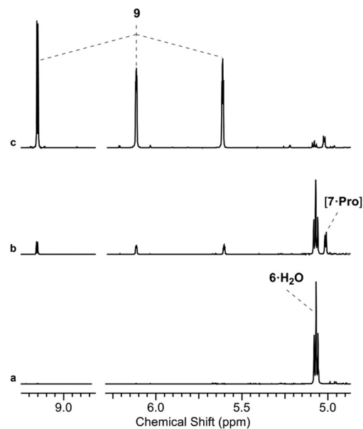
Fig. 2 Proline/phosphate co-catalysed reaction of glycolaldehyde phosphate and formaldehyde. 1 H NMR [400 MHz, noesygpprd, H 2 O/D 2 O (9 : 1)] spectra to show the reaction of glycolaldehyde phosphate ( 6 , 100 mM) with formaldehyde ( 8 , 100 mM) after 48 h at pH 7 and 40 °C: (a) in water; (b) with 50 mol% L-Pro in water; (c) with 50 mol% L-Pro in 500 mM phosphate.
