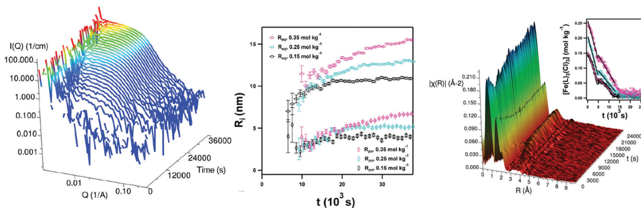
Fig. 19 (left) In situ small-angle neutron scattering data for iron oxide formation in a choline \text{Cl}:\text{Urea} DES. (middle) Results from fits to the SANS data, as a function of iron nitrate concentration, showing evolution in polar and equatorial iron oxide nanoparticle radius over time. (right) In situ EXAFS data and (inset) extracted Fe reaction kinetics, showing the same critical nucleation stage (5000 s) as the SANS data, and a change in rate at this point. Adapted with permission from the Royal Society of Chemistry. 312
