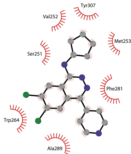
Fig. 27 Flat representation (generated using LigPlot+ from PDB ID 5CPR) showing contacts between compound 96 and active-site residues in SUV420H1. Hydrogen bonds are shown as dashed lines. The spokes arcs represent protein residues making non-bonded (hydrophobic) contacts with the compound.
