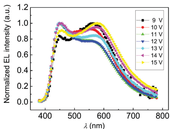
Fig. 23 Normalised EL spectra of a white OLED of 61 n = 2 under driving voltages of 9–15 V. Reproduced from ref. 173 with permission from Elsevier.
