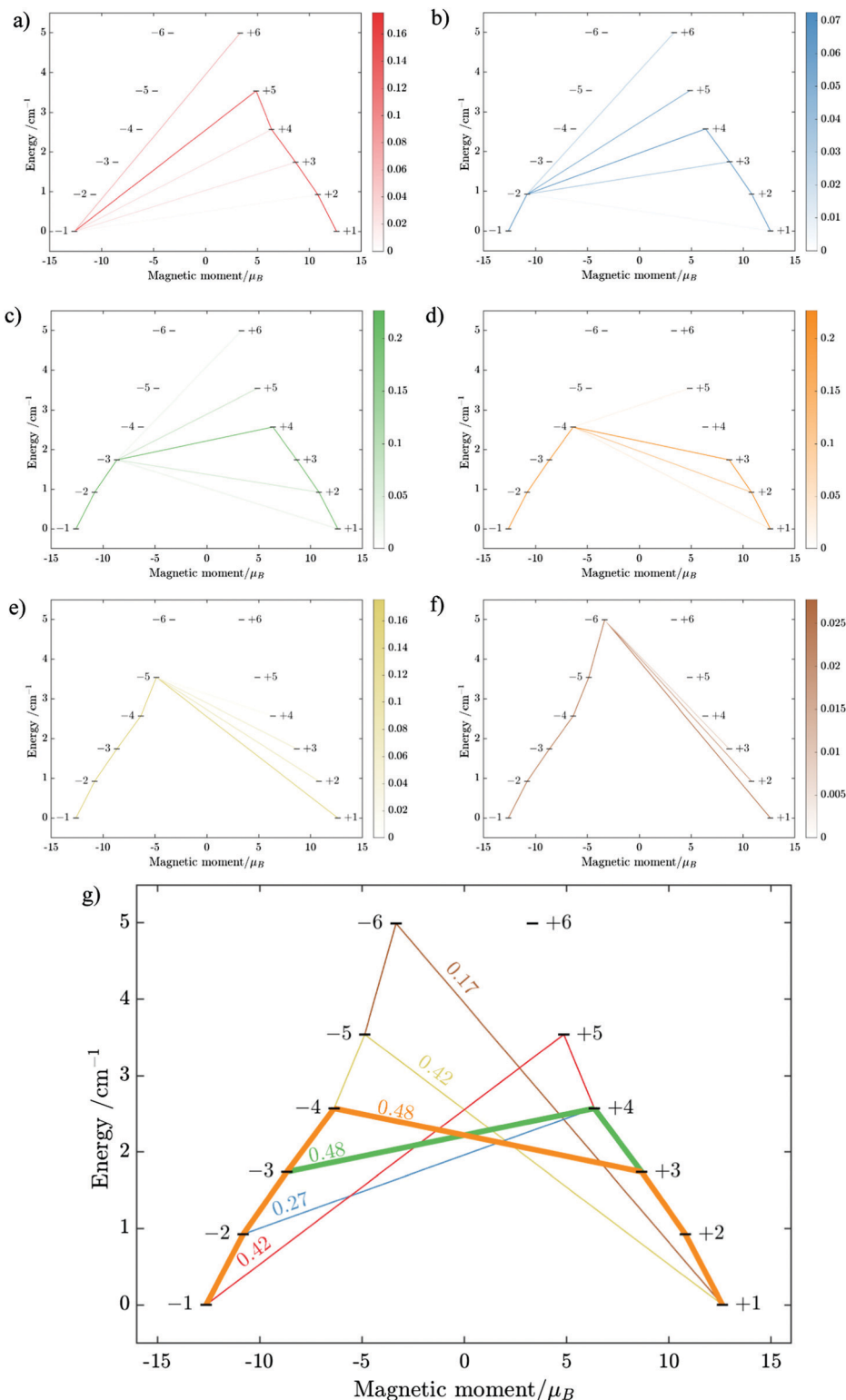
Fig. 10 Calculated relative transition conductance (non-horizontal lines) p_{ij} = p_{ij} = \frac{(E_j - E_i)^3}{e^{E_j/kT} - e^{E_i/kT}} |\mu_{ij}|^2 between any two localized states |i\rangle and |j\rangle of 6 lowest doublets involving in the magnetization relaxation at low temperature domain of [\text{Fe}^{\text{III}}\text{Tb}^{\text{III}}] complex ( 2 ), assuming that the whole population is initially prepared on the left side of the potential well. Here |\mu_{ij}| stands for average transition magnetic moment matrix element and taken from ab initio calculation, and T = 2 K is used for calculation of p_{ij} . Note that while relative transition conductance between states of different sides are shown with magnitude-dependent transparency, ones between states on the same side of the potential well are plotted without magnitude-dependent transparency. This is because population transition between states of the same side are much faster than ones between states of different sides, which is thus unimportant in determining the relaxation time of magnetization. Particularly, (a-f) p_{ij} for i = -1 \dots -6 respectively; (g) the largest p_{ij} for each i branch are plotted and compared to determined the dominant relaxation path (bold lines) from their corresponding p_{ij} . For [\text{Fe}^{\text{III}}\text{Tb}^{\text{III}}] at low temperature, the dominant paths are from |\pm 3\rangle \leftrightarrow |\mp 4\rangle .
