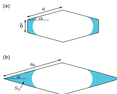
Fig. 5 Demonstration of the procedure to calculate the s^* in case (II). The meniscus position of s^* is shown in (a). For a diamond channel a_0 = a + b/(2 \sin \alpha) (b) with the saturation s_0^* , the position of the meniscus does not change in comparison with (a).
