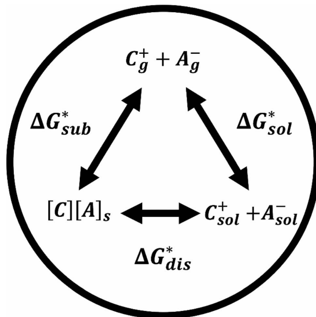
Fig. 2 Schematic representation of the thermochemical cycle for the dissolution of [cation][VBH] complexes. The free-energy of dissolution ( \Delta G_{dis}^* ) determines the solubility of the complex and results from the interplay between the free energy of sublimation ( \Delta G_{sub}^* ) and that of the stabilizing solute–solvent interactions in solution ( \Delta G_{sol}^* ).
