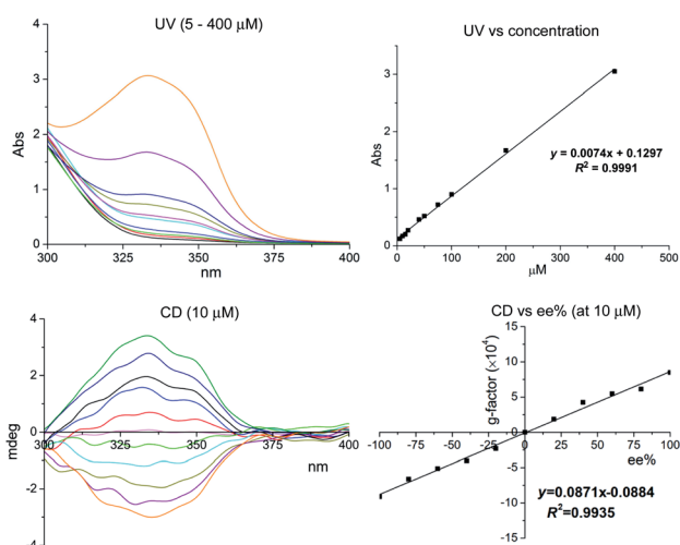
Fig. 3 Assaying \alpha AAs at varied concentrations. Standard conditions: 1.2 equiv. of 2 and 3e , 1 min for [\alpha\text{AA}] > 300 \mu\text{M} . Modified conditions: 5 equiv. and 1 min for 100–300 \mu\text{M} ; 20 equiv. and 3 min for 50–100 \mu\text{M} ; 100 equiv. and 3 min for 5–50 \mu\text{M} . See the ESI† for tests of Trp at 10 \mu\text{M} and Ala at 2 mM. (A) Test of Trp at normal concentration; a) all samples were diluted 6 times for the UV vs. concentration plot. The real measured concentration is 1/6 of the ones shown in the X axis. All samples (2 mM) were diluted 4 times for the CD vs. ee% plot, measured at 0.50 mM. (B) Plots of CD vs. ee% of selected \alpha AA. (C) Test of Ala at low concentration; b) assaying samples were measured without dilution. The g-factor was the average of four measurements.
