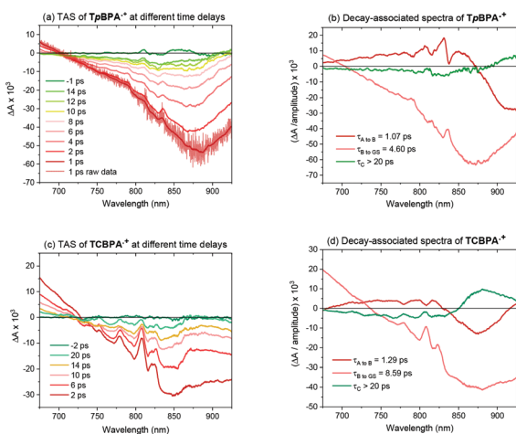
Fig. 8 Transient absorption and decay-associated spectra of TPA + s.
