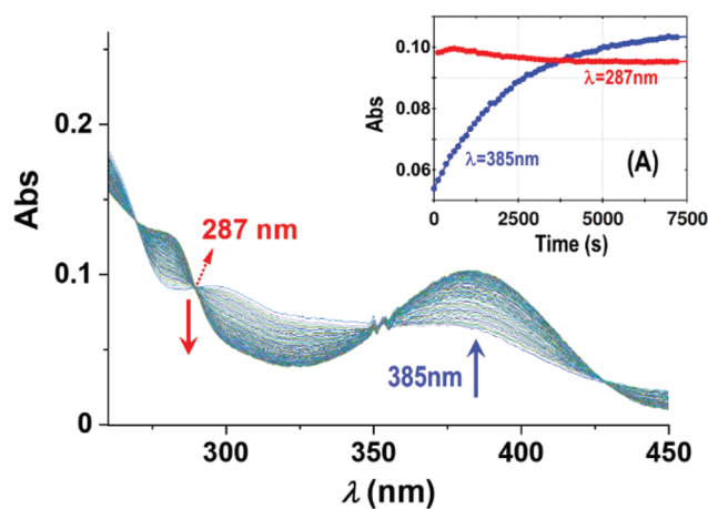
Fig. 6 Absorbance changes of 1-OH 2 (16 \mu\text{M} ) around the isobestic point (287 nm) with time in the presence of PPI (10 equiv.; 0.16 mM) at pH 7.35 ([Tris buffer] = 10 mM) and 12 ^{\circ}\text{C} illustrating the presence of earlier reactions. Inset (A): L.S. fits of Abs vs. time at 287 nm (red) and 385 nm (blue), respectively, showing the small absorbance changes of the first reactions (induction period) and underlining the small absorbance changes therewith, not influencing the individual fits and kinetic data as illustrated in the k_{\text{obs}} vs. [\text{PPI}]_{\text{tot}} graph in Fig. 3 and 5.
