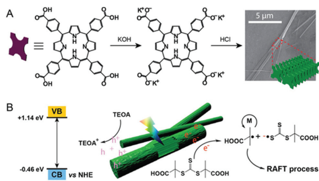
Fig. 15 Self-assembly of rod-like SA-TCPP and its use in PET-RAFT polymerization. Reproduced from ref. 153 with permission from Wiley-VCH Verlag GmbH & Co. KGaA, Weinheim, copyright 2020.
