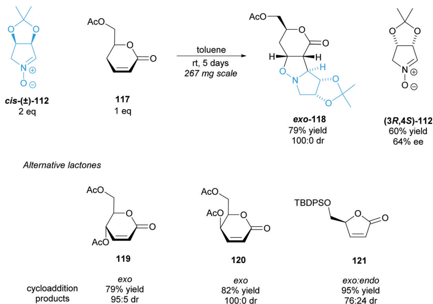
Scheme 30 1,3-dipolar cycloaddition of racemic nitron 112 to various lactones reported by Chmielewski et al.
