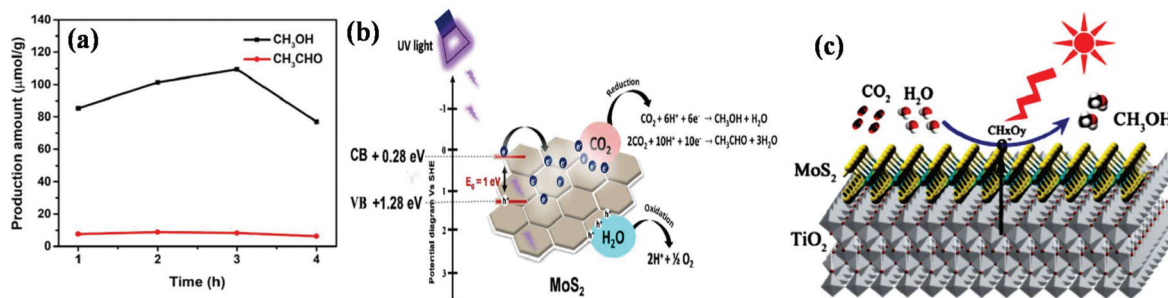
Fig. 14 (a) Rate of \text{CO}_2 reduction by \text{MoS}_2 sheets in 0.5 M \text{NaHCO}_3 and (b) schematic representation of the mechanistic pathway for photocatalytic \text{CO}_2 reduction over \text{MoS}_2 sheets. Reproduced with permission. 173 (c) Schematic illustration of the photoreduction of \text{CO}_2 to \text{CH}_3\text{OH} in the \text{MoS}_2/\text{TiO}_2 heterostructure. Reproduced with permission. 170
