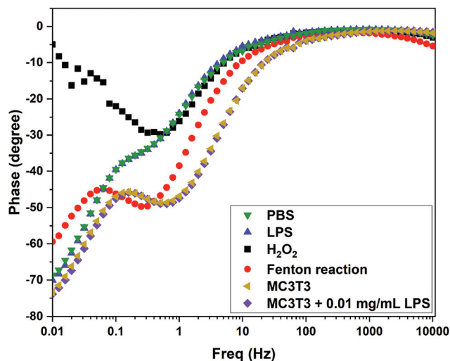
Fig. 7 Phase shifts in Bode plots for the electrochemical impedance spectroscopy (EIS) results obtained with the 0.64 wt% Ce/Carbon-modified electrode in the presence of PBS, LPS, \text{H}_2\text{O}_2 , Fenton reaction, MC3T3, and MC3T3 + LPS (additional induced oxidative stress).
