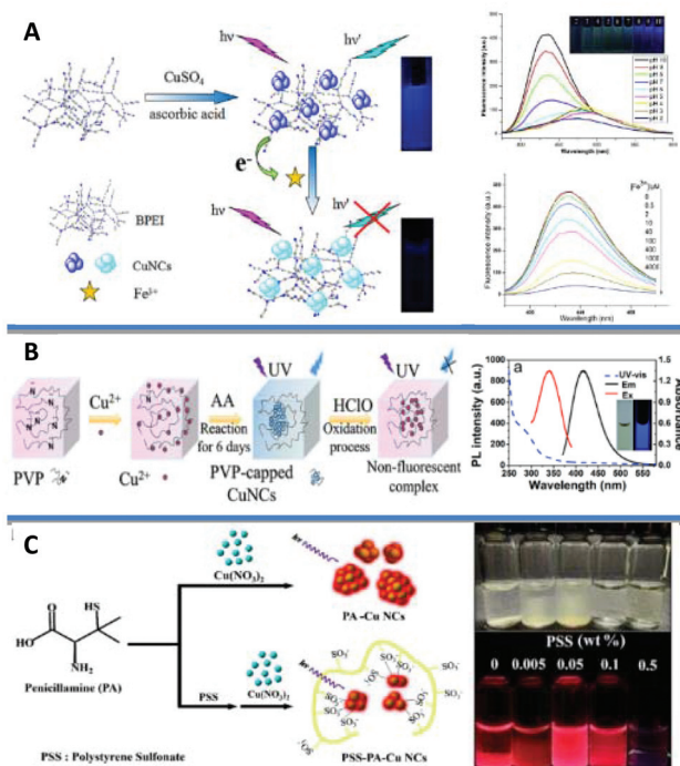
Fig. 2 (A) Synthesis strategy for the BPEI-CuNCs, their stability under varying pH and the mechanism of the branched polyethyleimine (BPEI)-CuNCs probe for \text{Fe}^{3+} sensing. Reprinted with permission from ref. 30. Copyright 2015 Elsevier. (B) Schematic diagram of PVP-capped CuNCs (on the left) and UV-vis absorption, emission, and excitation fluorescence spectra of the probe CuNCs at pH = 6.2 in 50 mM phosphate buffer (PB) (on the right). Inset: Photograph of CuNCs probe in buffer under daylight (left) and UV-light ( \lambda = 365 nm, right), respectively. Reprinted with permission from ref. 34. Copyright 2020 American Chemical Society. (C) A scheme depicting a plausible mechanism for the synthesis of PSS-stabilized penicillamine (PA)-CuNCs and the photographs of the PSS-PA-CuNCs synthesized under different concentrations of PSS, from 0.005 to 0.5 wt%. Adapted with permission from ref. 35. Copyright 2016 Springer Nature.
