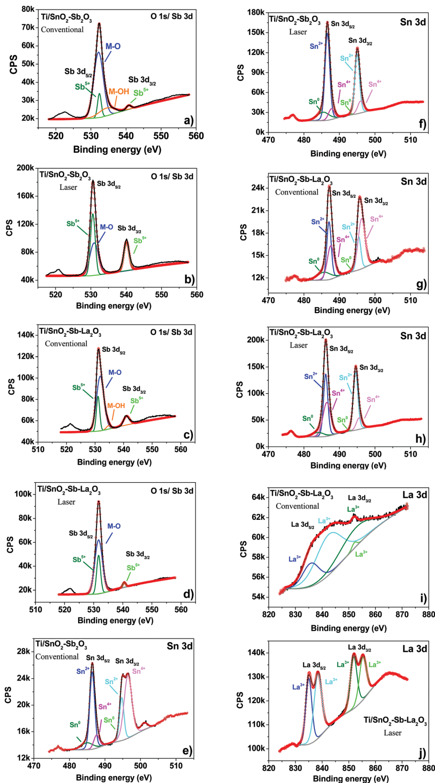
Fig. 4 High-resolution XPS spectrum of O 1s/Sb 3d, Sn 3d and La 3d for Ti/SnO 2 -Sb 2 O 5 electrodes (a and e) conventional, (b and f) laser and Ti/SnO 2 -Sb-Lao 3 electrodes. (c, g and i) Conventional and (d, h, and j) laser.
