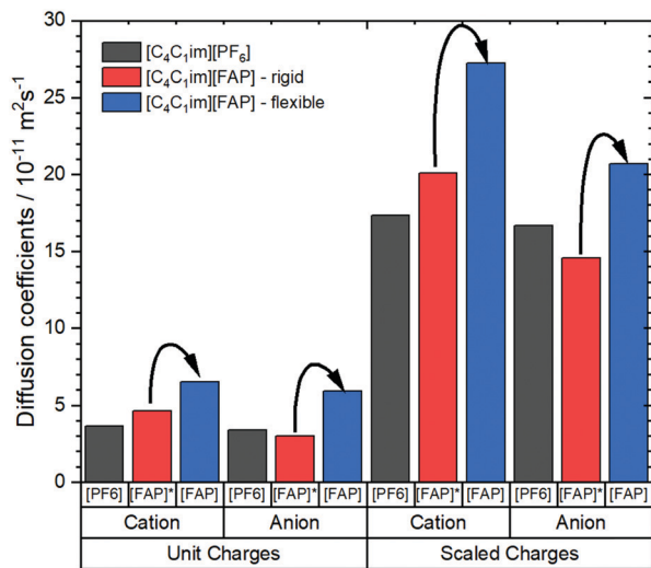
Fig. 14 Diffusion coefficients of [\text{C}_4\text{C}_1\text{im}][\text{PF}_6] and [\text{C}_4\text{C}_1\text{im}][\text{FAP}] obtained from molecular dynamics simulations. 191 The simulations were set up with scaled vs. unit charges and flexible vs. rigid anions. Arrows indicate the increase in diffusion when the FAP anion is allowed to be flexible, regardless if charges are scaled or not.
