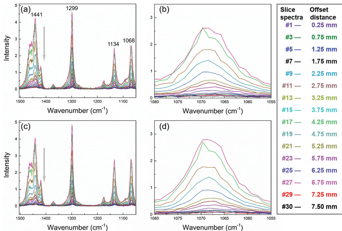
Fig. 3 SORS line-mapped spectra of the 303 \mu\text{m} LDPE packing in the 1504–1050 (a) and 1080–1055 \text{cm}^{-1} ranges (b) and the 282 \mu\text{m} MDPE packing in the 1504–1050 (c) and 1080–1055 \text{cm}^{-1} (d) ranges.
