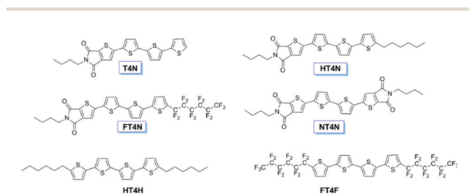
Fig. 3 Molecular structures of the quaterthiophene derivatives including TI ended compounds. Reprinted with permission from Chem. Mater. , 2013, 25 (5), 668–676. Copyright (2013) American Chemical Society.
