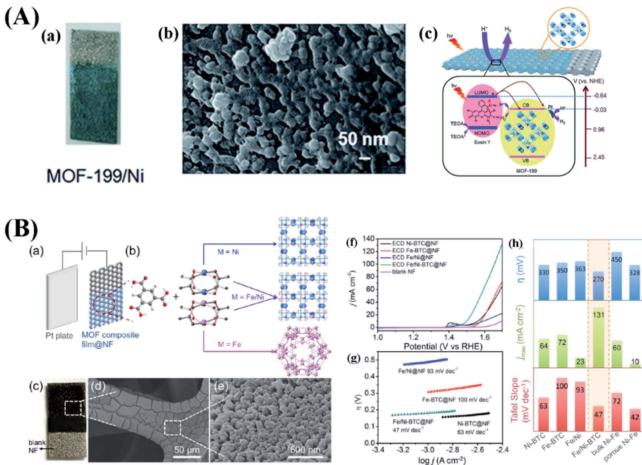
Fig. 5 (A) (a) Optical photograph and (b) SEM image of the MOF-199/Ni film prepared by electrodeposition with (c) the schematic of the eosin-Y sensitized photocatalytic process on the MOF-199/Ni film. Reproduced with permission from ref. 57. Copyright 2016, the Royal Society of Chemistry. (B) (a) ECD process of Fe/Ni-BTC MOF thin films. (b) Design and synthesis of Fe/Ni-BTC MOFs. (c) Optical image, (d) scanning electron microscopy (SEM) image, and (e) higher-magnification image of Fe/Ni-BTC@NF. (f) LSV curves of ECD Ni-BTC@NF, ECD Fe-BTC@NF, ECD Fe/Ni@NF, ECD Fe/Ni-BTC@NF, and NF measured at 2 \text{ mV s}^{-1} . (g) Tafel plots of ECD Ni-BTC@NF, ECD Fe-BTC@NF, ECD Fe/Ni@NF, and ECD Fe/Ni-BTC recorded at 1 \text{ mV s}^{-1} . (h) Comparison of ECD Ni-BTC, ECD Fe-BTC, ECD Fe/Ni, ECD Fe/Ni-BTC, bulk Ni-Fe oxides, and porous Ni-Fe oxides. Reproduced with permission from ref. 96. Copyright 2016, American Chemical Society.
