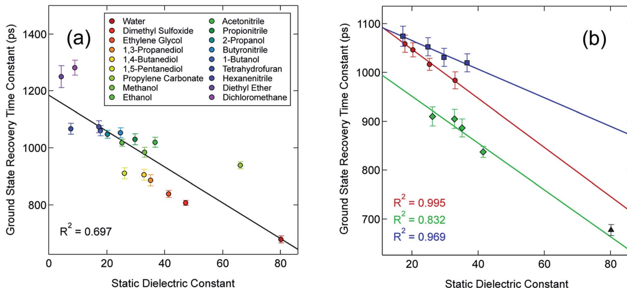
Fig. 2 (a) Time constants for ground state recovery of [\text{Fe}(\text{bpy})_3]^{2+} following ^1A_1 \rightarrow ^1\text{MLCT} excitation at 550 nm as a function of the static dielectric constant of the solvent. (b) A subset of the data from (a) grouped according to solvent type, specifically alcohols (red circles), diols (green diamonds), and nitriles (blue squares). The black triangle corresponds to data acquired in aqueous solution (a typical solvent choice in the literature for this complex), but is not included in any of the fits for reasons to be discussed later.
