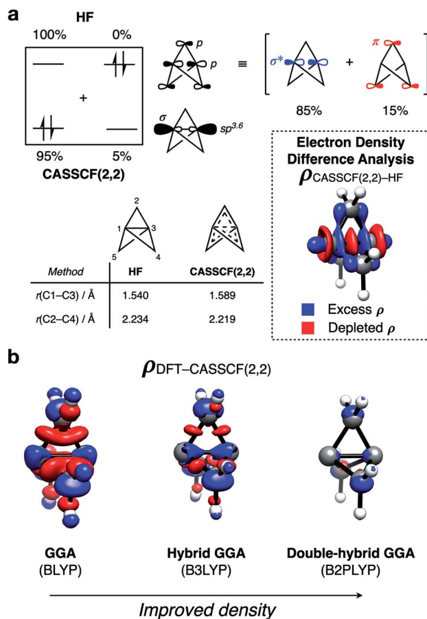
Fig. 2 (a) Top: populations and symmetries of MOs in the (2,2) active space with their corresponding atomic orbital composition. Bottom left: effect of \sigma – \pi -delocalization on key geometric features of 1 . Inset: [CASSCF(2,2)]–[RHF] electron density difference plot for 1 , isovalue = 0.002 a.u. (b) DFT electron density difference plot for 1 : [BLYP]–[CASSCF(2,2)] (left), [B3LYP]–[CASSCF(2,2)] (center), [B2PLYP]–[CASSCF(2,2)] (right); isovalue of 0.01 a.u. Geometry optimized at CASSCF(2,2). All calculations use the def2-QZVPP basis set.
