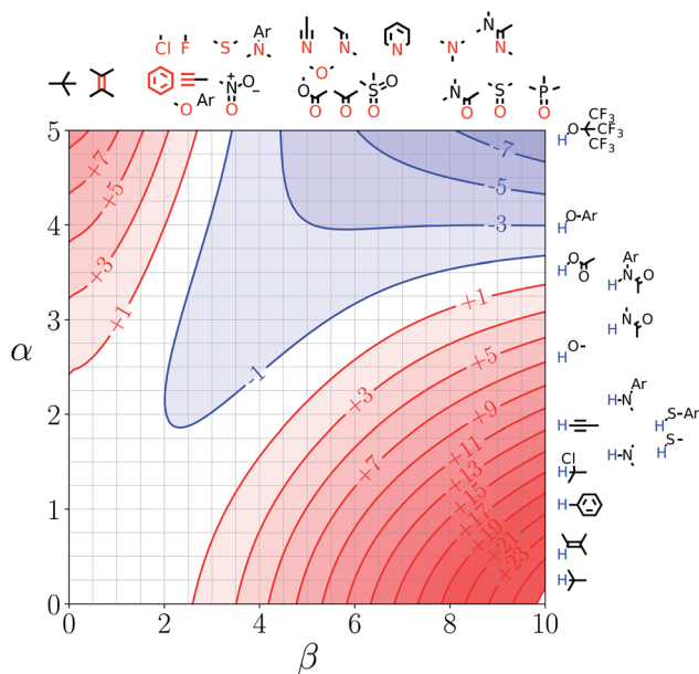
Fig. 7 FGIP for the interaction of two solutes in formic acid at 298 K ( \Delta G_{\text{FGI}} in \text{kJ mol}^{-1} ). The solute–solute interactions in the blue region, and unfavourable in the red region.
