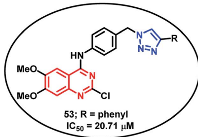
Designing strategy for Quinazoline-triazole hybrids
