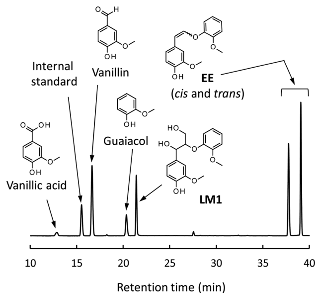
Fig. 4 HPLC chromatogram of the reaction mixture obtained after the degradation of LM2 (5 mg) in 1.25 \text{ mol L}^{-1} Bu 4 NOH aq. (1.0 mL) under air for 1 h.
