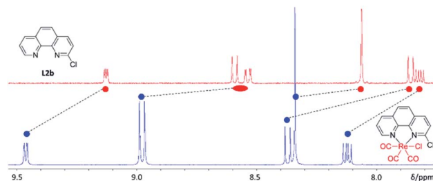
Fig. 6 Example of the downfield chemical shifts in ^1\text{H-NMR} aromatic signals observed when complexing L2b (top, red) with [\text{Re}(\text{CO})_3\text{Cl}] to form [\text{Re}(\text{L2b})(\text{CO})_3\text{Cl}] (bottom, blue). The shifts suggest electron withdrawal from the \pi -aromatic system which likely facilitates nucleophilic substitution for [ ^{18}\text{F} ]fluoride.
