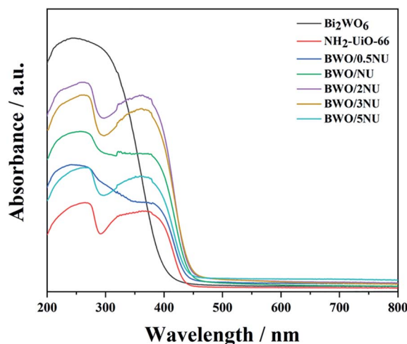
Fig. 8 UV-vis DRS spectra of as-prepared samples.
