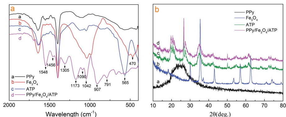
Fig. 1 IR (a) and XRD (b) spectra of PPy, \text{Fe}_3\text{O}_4 , ATP and \text{PPy}/\text{Fe}_3\text{O}_4/\text{ATP} composite.
