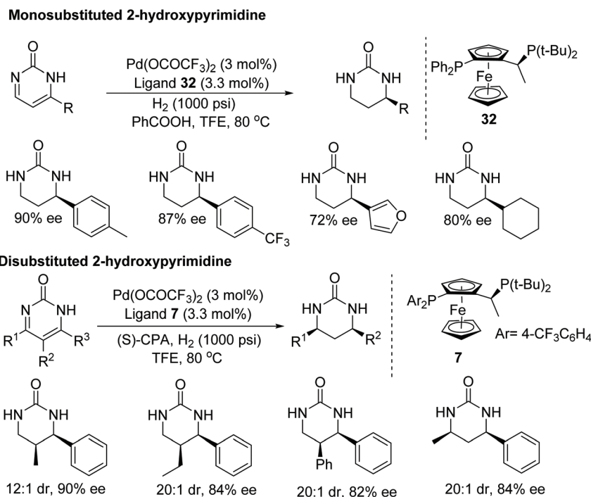
Fig. 43 Palladium catalysed AH of mono- and disubstituted 2-hydroxypyrimidines.
