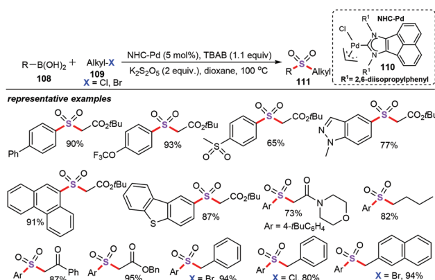
Scheme 41 Palladium-catalyzed alkylsulfonation of boronic acids with alkyl halides.
