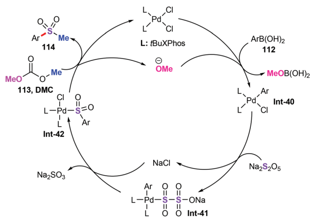
Scheme 43 Plausible mechanism for the three-component sulfonation reaction.
