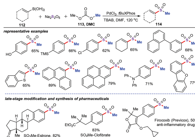
Scheme 42 Palladium-catalyzed three-component cascade sulfonation reaction.
