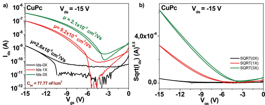
Fig. 7 (a) Comparison of OFET devices with three different purity grades of copper phthalocyanine semiconductor: unpurified (0× in graph legend), one time purified (1× in graph legend) and three times purified, respectively (3× in graph legend); (b) the \sqrt{I_{ds}} vs. V_{gs} of the three purity grades presented in panel (a).
