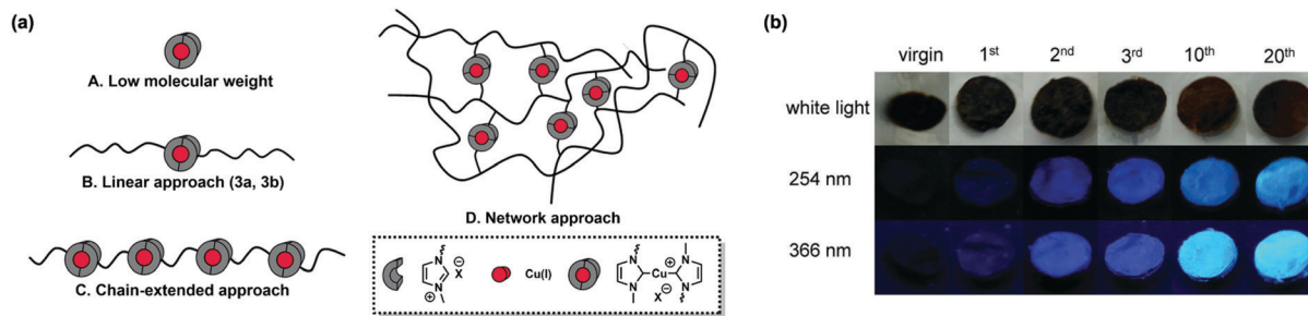
Fig. 4 (a) Different architectures of mechanocatalysts: (A) low molecular weight, (B) linear, (C) chain-extended, and (D) network-based mechanocatalysts. (b) Photos of investigated samples (linear mechanocatalyst 3b , 3-azido-7-hydroxycoumarin, and phenylacetylene embedded into a high molecular weight pTHF matrix) before and after the 1st, 2nd, 3rd, 10th, and 20th compression cycle with a hydraulic press (0.74 GPa) visualized under white or UV light (254 or 366 nm), respectively. Reproduced with permission. 41 Copyright 2018, John Wiley and Son.
