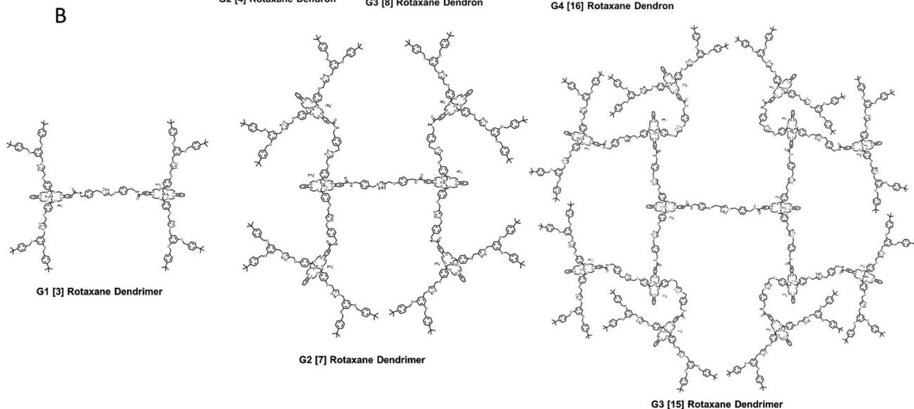
Fig. 14 Leung's Type III-B rotaxane dendrimers. (Copyright: Nature Publishing Group.)
