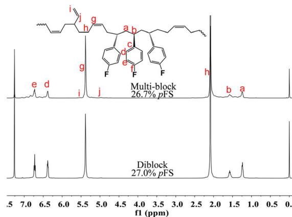
Fig. 5 ^1\text{H} NMR spectra of multi-block and diblock poly( p -FS-BD) (500 MHz, \text{CDCl}_3 , 25 ^\circ\text{C} ).
