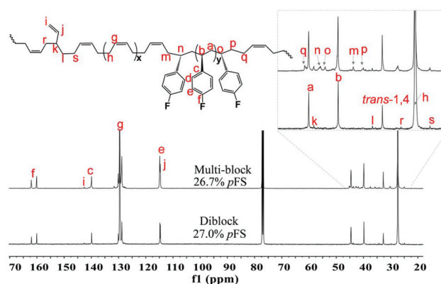
Fig. 6 ^{13}\text{C} NMR spectra of multi-block and diblock poly( p -FS-BD) (125 MHz, \text{CDCl}_3 , 25 ^\circ\text{C} ).
