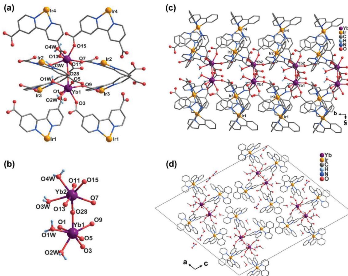
Fig. 3 (a) The building unit of the structure of \text{Ir}_4\text{Yb}_2 . The ppy ligands are omitted for clarity. (b) Coordination environments of the Yb III ions. (c) The double-chain structure of the compound \text{Ir}_4\text{Yb}_2 . (d) Packing diagram of the structure of \text{Ir}_4\text{Yb}_2 viewed along the b-axis. All H atoms except those attached to the oxygen atoms are omitted for clarity.
