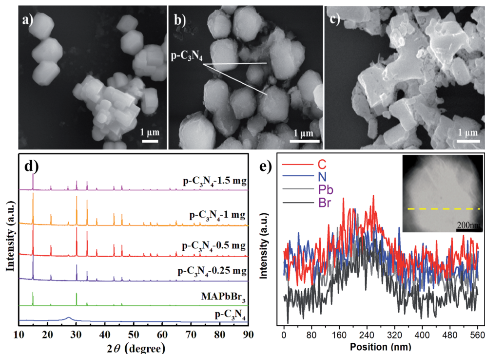
Fig. 2 (a–c) SEM images of MAPbBr 3 /p-g-C 3 N 4 -0, -1.0, and -1.5 mg samples, respectively. (d and e) The corresponding XRD patterns and EDS line scan image of an individual MAPbBr 3 microcrystal encapsulated nanosheet.
