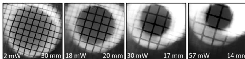
Fig. 5 Images of the test grid obtained with the solutocapillary lens (50% ethylene glycol, 1 \mu\text{l} ) at different laser beam powers.
