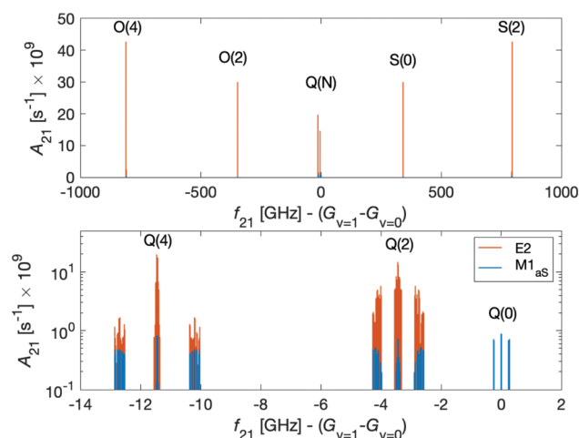
Fig. 10 Einstein A coefficients of E2 (red lines) and M1_{as} (blue lines) transitions of the O( N = 2, 4 ), Q( N = 0, 2, 4 ) and S( N = 0, 2 ) branches of the fundamental vibrational transition |\nu = 0, N\rangle \rightarrow |\nu' = 1, N'\rangle . The magnetic field was assumed to be 5 G. The lower panel shows a magnification of the spectrum in the region of the Q branch.
