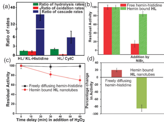
Fig. 4 (a) Ratios of the rates of HL to KL -histidine systems and HL to CytC for hydrolysis, oxidation and cascade reactions. Residual activities of (b) free hemin-histidine and hemin-HL systems challenged by inhibitor NiBr 2 , (c) delayed addition of H 2 O 2 to the free histidine hemin and hemin-HL systems, (d) percentage change in activity when MPA was added to HL or only histidine without hemin, and after 10 min delay, hemin was added. [Hemin] = 0.01 mM, [ HL ] = 1 mM, [histidine] = 1 mM, [H 2 O 2 ] = 30 mM.
