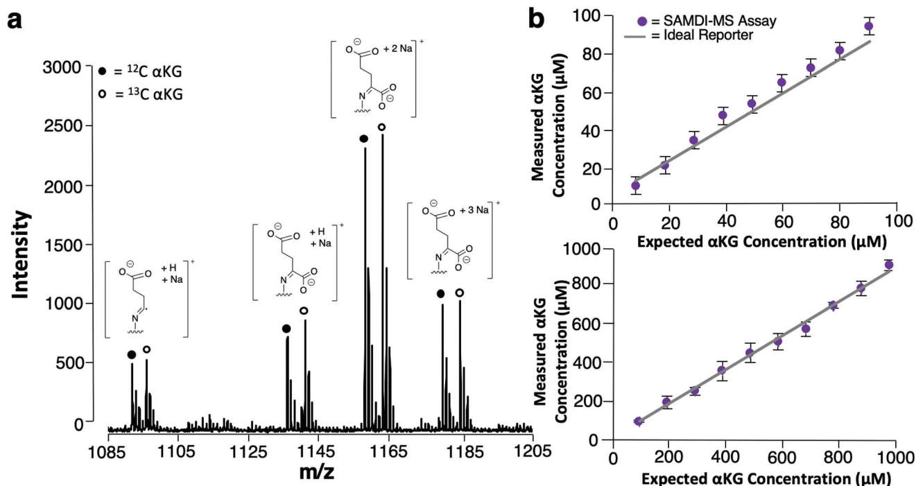
Fig. 3 (a) Representative SAMDI-MS spectrum of a 1 mM ^{12}C and 1 mM ^{13}C \alpha KG solution displaying the sodium adduct of the \alpha -cleavage product at m/z = 1091 ( ^{12}C ) and m/z = 1095 ( ^{13}C ), the sodium adduct at m/z = 1135 ( ^{12}C ) and m/z = 1140 ( ^{13}C ), the double sodium adduct at m/z = 1157 ( ^{12}C ) and m/z = 1162 ( ^{13}C ) and the triple sodium adduct at m/z = 1179 ( ^{12}C ) and m/z = 1184 ( ^{13}C ). (b) Sensitivity plots comparing measured \alpha KG concentration to known \alpha KG concentration for solutions ranging from 10 to 90 \mu M (top) and from 100 \mu M to 1 mM (bottom). Data are expressed as mean \pm standard deviation, with n = 8 –10 technical replicates per solution.
