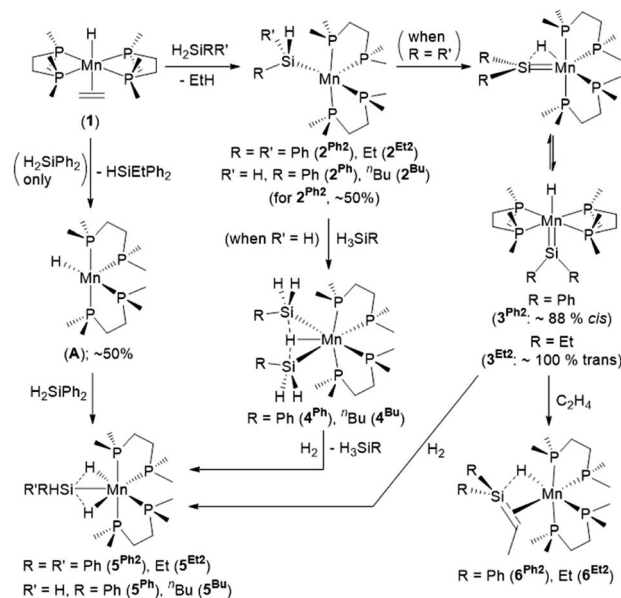
Scheme 1 Reactions of [(dmpe)_2MnH(C_2H_4)] ( 1 ) with primary and secondary hydrosilanes to generate silylene-hydride ( 3^{R_2} ) and disilyl hydride ( 4^R ) complexes respectively, reactions of the latter two complexes with H_2 to generate isostructural silyl dihydride complexes ( 5^{R_2} or 5^R respectively), and reaction of silylene hydride complexes 3^{R_2} with ethylene to generate silene hydride complexes ( 6^{R_2} ). 32,35,36 Only one isomer is shown for 2 , 5 , and A .
