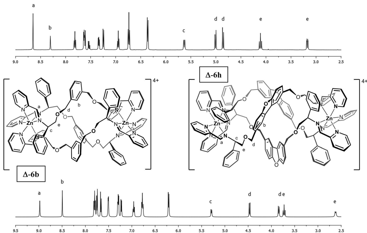
Fig. 1 ^1\text{H-NMR} spectra of metallohelices \Delta\text{-6b} and \Delta\text{-6h} (500 MHz in d^5 -acetonitrile at 298 K). Note the presence of single diastereomers and the unusual chemical shifts of the nuclei at position b in both cations.
